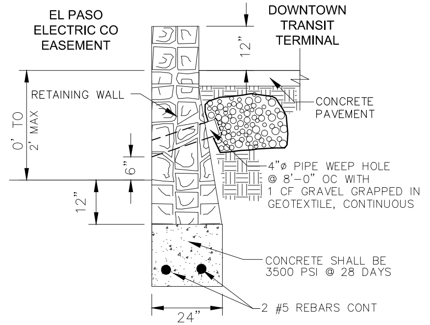
RETAINING WALL DETAIL NTS
