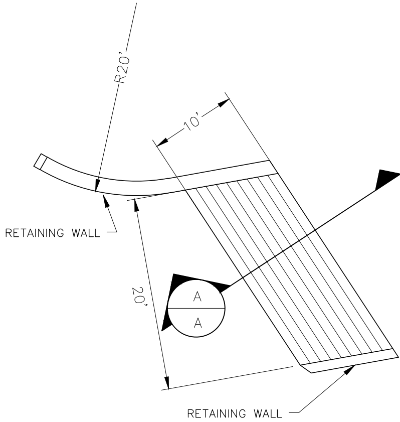
RAMP PLAN VIEW NTS
